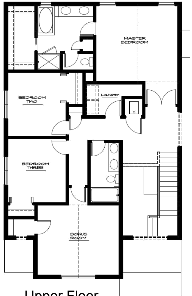
Upper Floor
